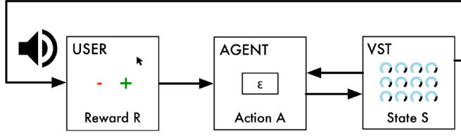
Fig. 4. Our RL agent prototype. Users can only provide feedback to the agent, which acts on hidden VST parameters.
